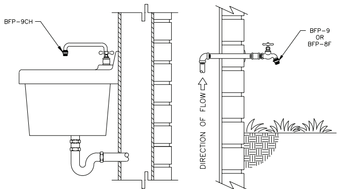
TYPICAL SERVICE SINK INSTALLATION
